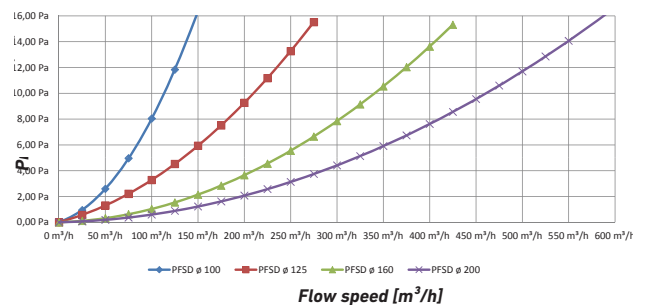
Pressure loss
