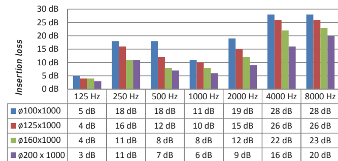
Insertion loss PFSD Ø 100 - 202 l = 1000
