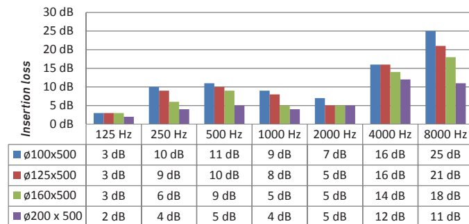
Insertion loss PFSD Ø 100 - 200 l = 500
